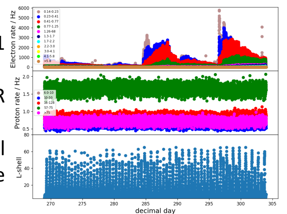
L-shell, electron and proton rates measured by satellite ns53 on 26/09 – 31/10/2010
