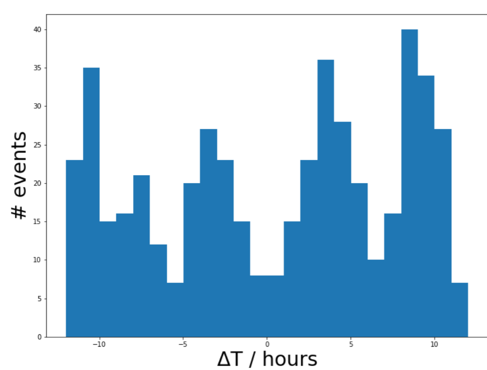
Temporal correlation histogram for satellite ns54
