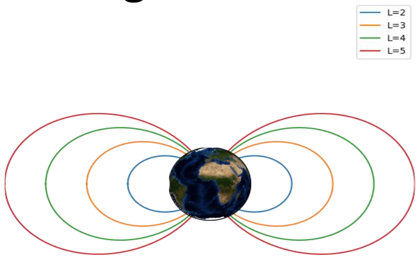
L-shell distribution around the Earth
