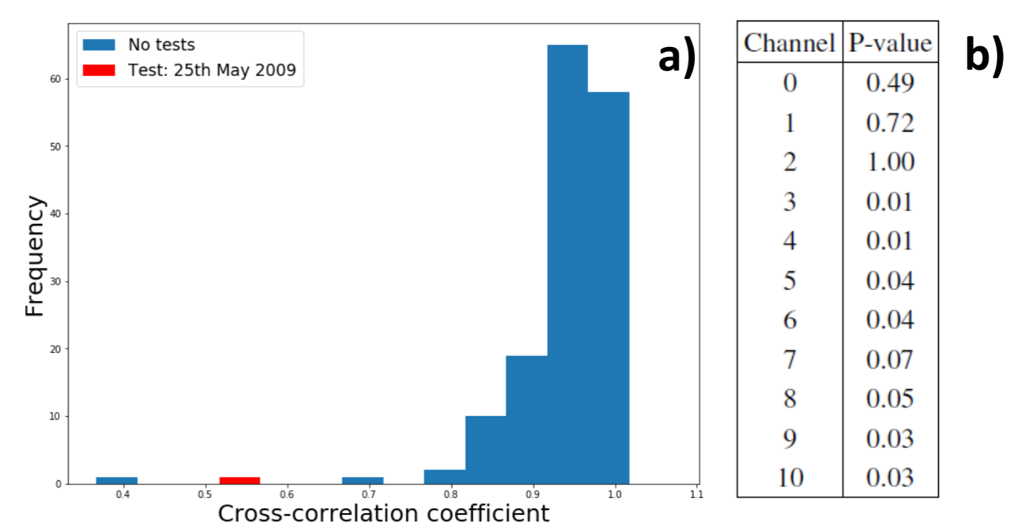
a) Cross – correlation histogram for channel 2 with channel 4; b) Table of p-values for DPRK's test from 25th May 2009
